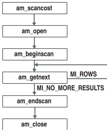
Figure 4-13. Processing a SELECT Statement Scan
