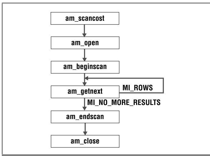
Figure 4-13 Processing a SELECT Statement Scan
