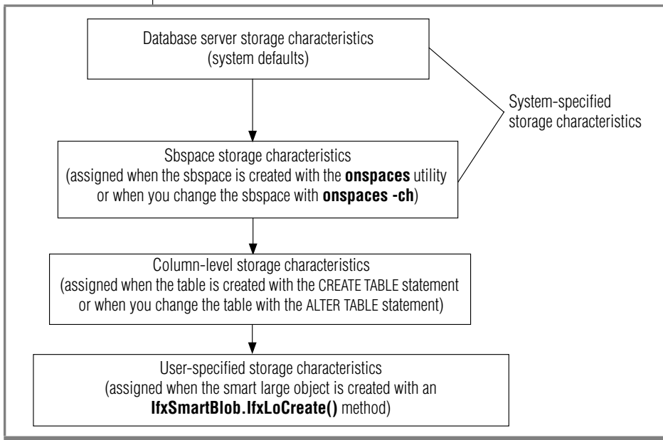
Figure 4-3 Storage- Characteristics Hierarchy
