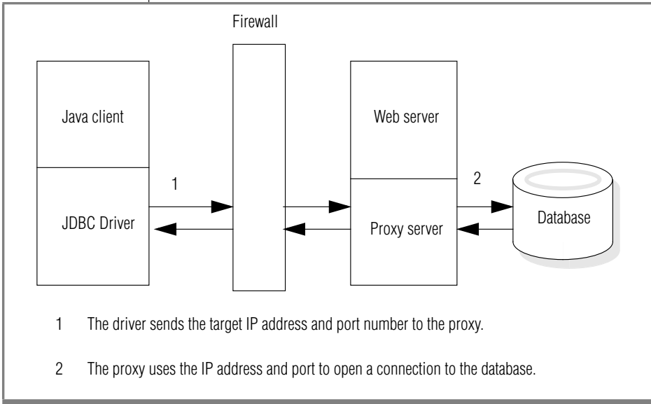
Figure 2-1 Connecting Through a Firewall
