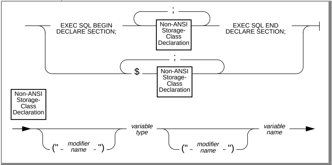
Figure 1-31 ESQL/C Syntax for Non-ANSI Storage-Class Specifiers
