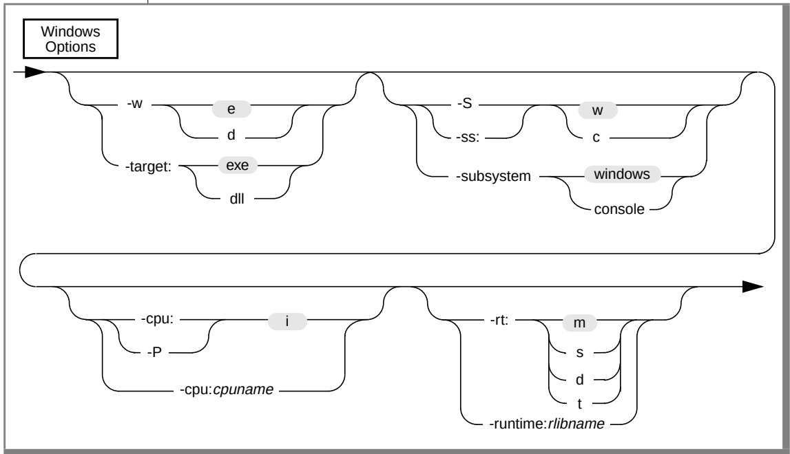
Figure 1-27 Windows Environment Options available to esql
