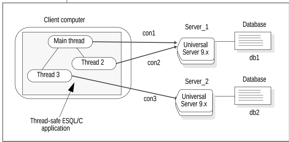
Figure 13-4 Concurrent Connections in a Thread-Safe ESQL/C Application
