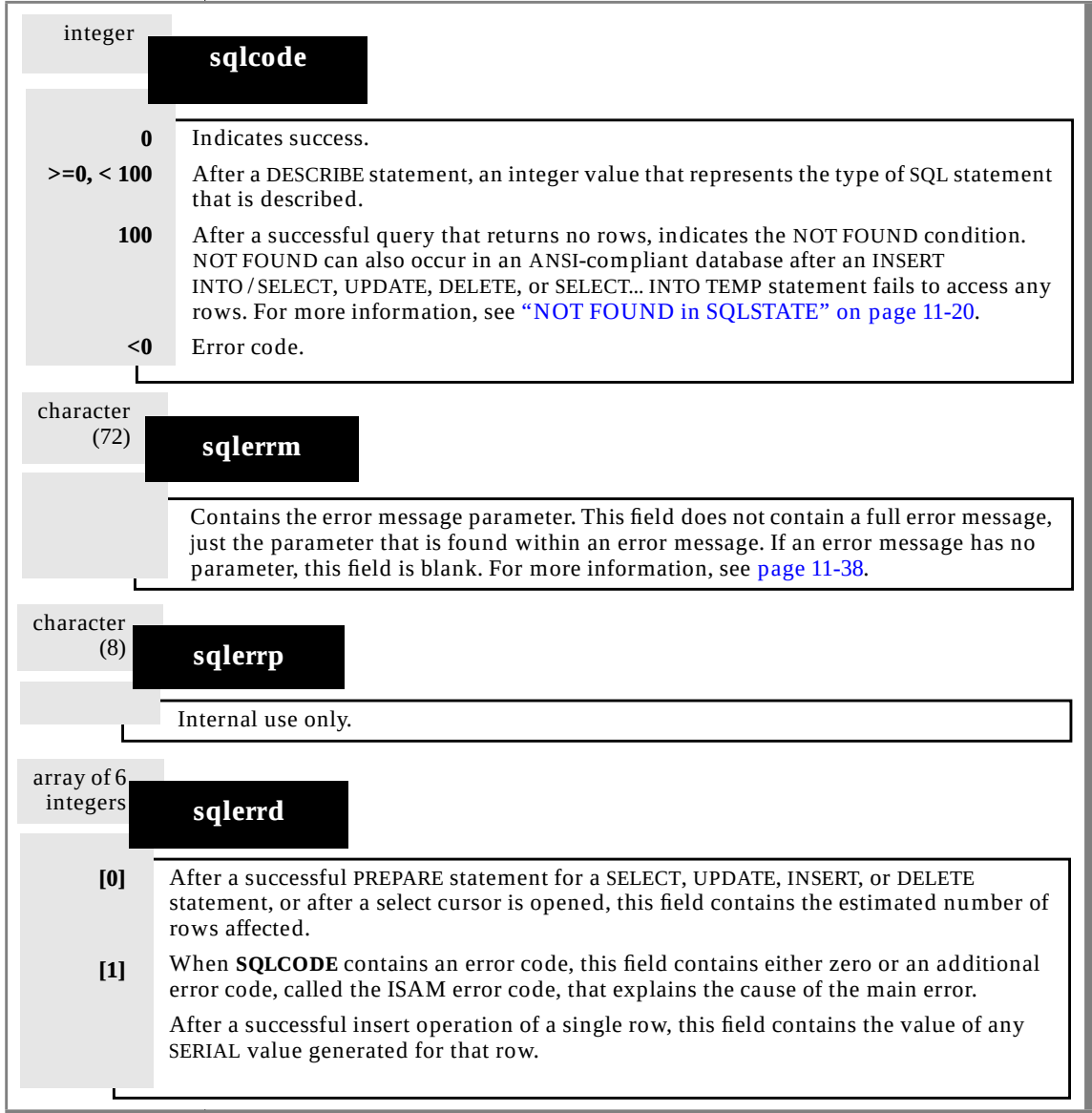
Figure 11-14 Fields of the sqlca Structure
