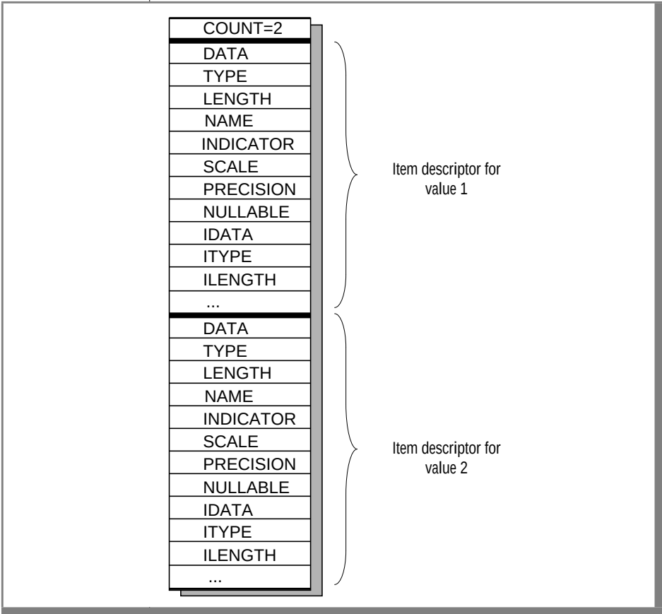
Figure 15-1 Schematic That Shows System-Descriptor Area for Two Values
