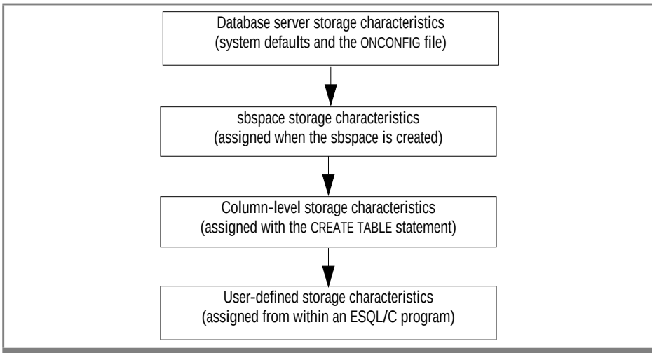
Figure 7-3 Inheritance Hierarchy for Storage Characteristics
