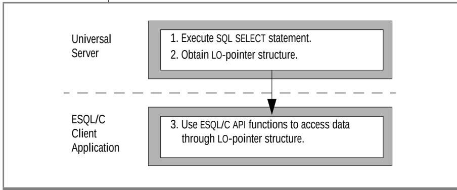
Figure 7-5 Transferring Smart-Large-Object Data from Database Server to Client Application
