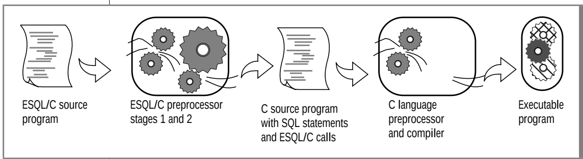
Figure 1-1 Relationship Between INFORMIX-ESQL/C and C
