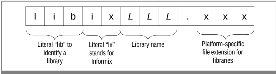
Figure 13-3 Format of an Informix Shared-Library Name
