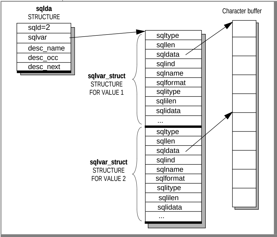
Figure 15-4 Schematic That Shows sqlda Structure for Two Values
