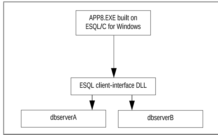
Figure 12-8 One Application That Uses Connections to More Than One Database Server at the Same Time
