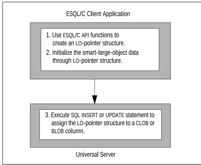
Figure 7-4 Transferring Smart-Large-Object Data from Client Application to Database Server
