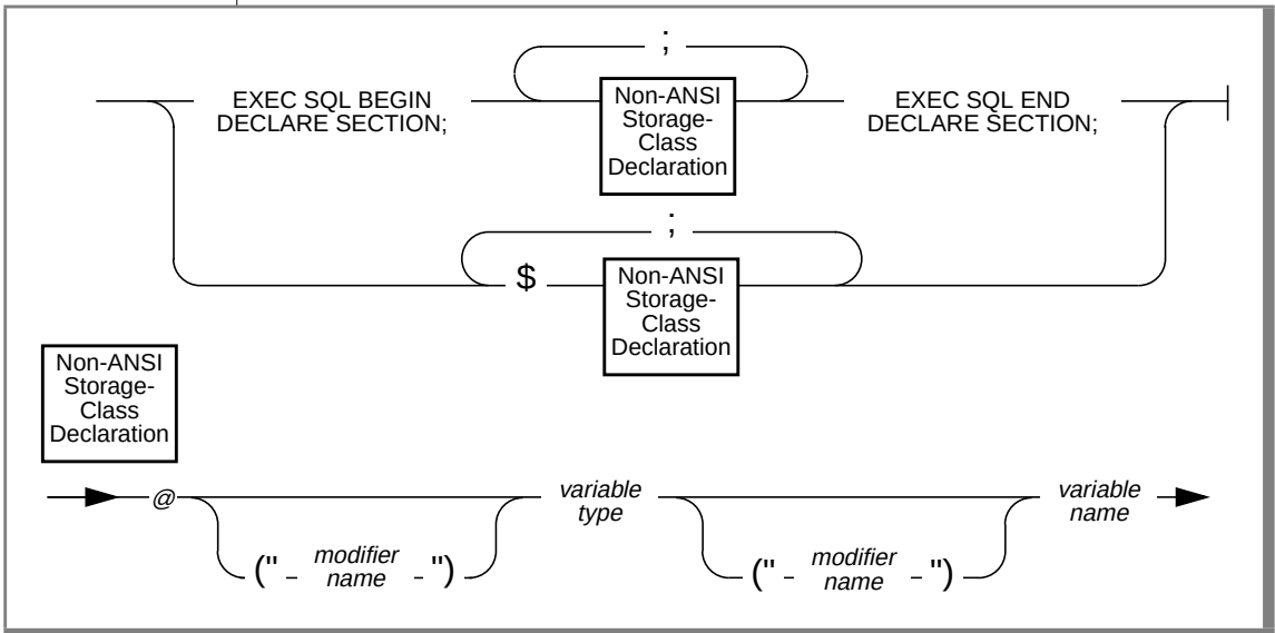
Figure 1-14 ESQL/C Syntax for Non-ANSI Storage-Class Specifiers
