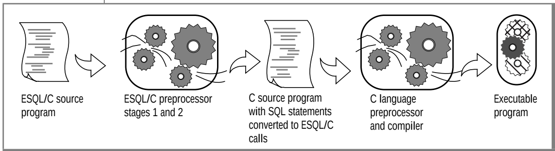
Figure 2-1 Relationship Between INFORMIX-ESQL/C and C
